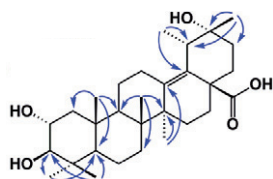
Fig. 1 - Experimental correlations in NOESY and HMBC observed in compound 1.
