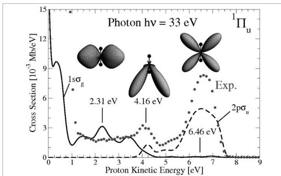
Figure 2. ^1\Pi_u proton kinetic energy distribution (KED) in the dissociative ionization of H_2 for protons detected at 90^\circ with respect to the laser polarization axis and photon energy 33 eV. Solid line: contribution from the ^2\Sigma_g^+(1s\sigma_g) ionization channel; dashed line: contribution from the ^2\Sigma_u^+(2p\sigma_u) ionization channel; dots: experimental data from Ref. [1] must be compared with the sum of both contributions. Correct electron angular distributions (EADs) are in display for three selected proton energies. In the EADs the laser polarization vector is perpendicular to the molecular axis within the plane of the figures and the proton is pointing upwards. Mb stands for Megabarn (1 barn = 1024 cm 2 ).
