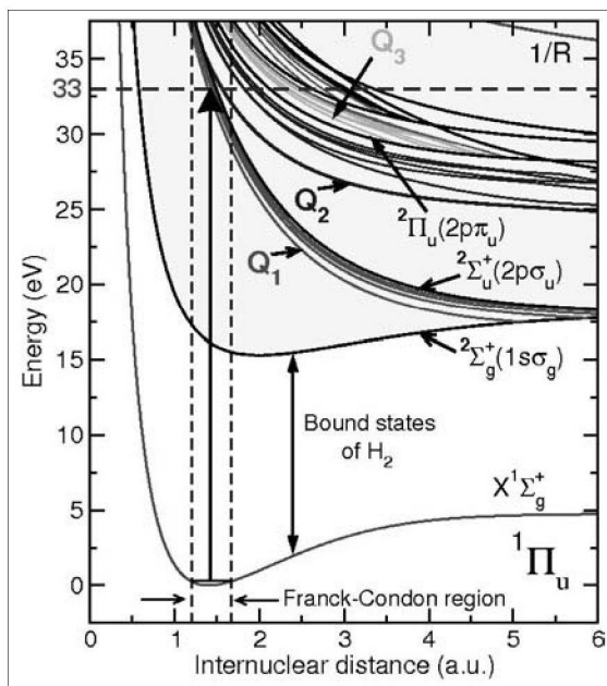
Figure 1. Potential energy curves of H_2 and H_2^+ . The lowest two series of Q_1 and Q_2 autoionizing doubly excited states of H_2 with ^1\Pi_u symmetry are included. The vertical arrow indicates a one-photon transition of 33 eV from the ground state energy level within the Franck-Condon region.
