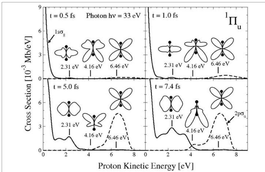
Figure 4. Time evolution for the ^1\Pi_u proton kinetic energy distribution (KED) and for the electron angular distributions (EAD) at three proton energies in the dissociative ionization of H_2 mediated by a laser pulse with duration of T = 10 fs and photon energy \omega = 33 eV. The propagation time for each snapshot is indicated. Results for t = T = 10 fs are those included in Figure 3.
