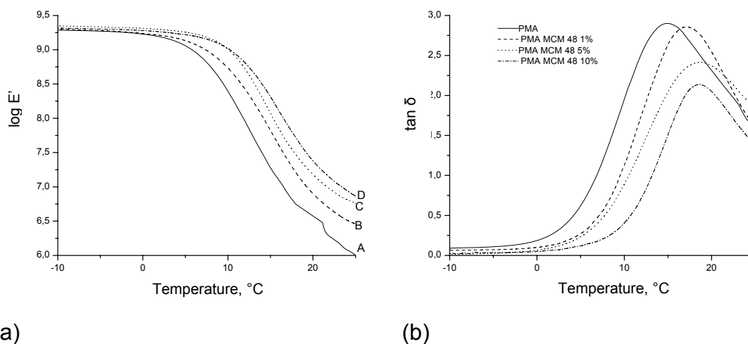
Fig. 6. (a) DMA results; A) \log E' vs. temperature; (b) \tan \delta vs. temperature. Silica contents: A) PMA, B) PMA MCM-48 1, C) PMA MCM-48 5, D) PMA MCM-48 10.
