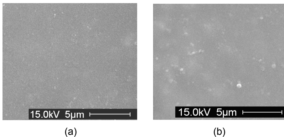
Fig. 3. Nanohybrid morphology. (a) PMA MCM-48 5, (b) PMA MCM-48 10.
