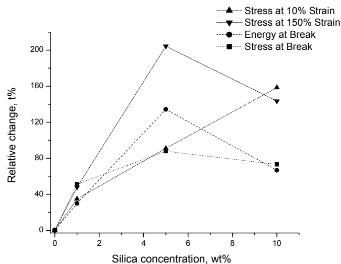
Fig. 7. Relative changes in the tensile properties at different silica concentrations.
