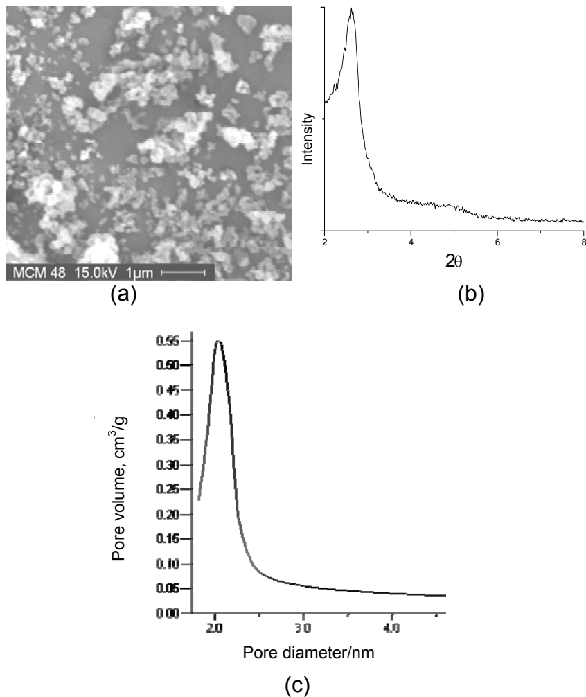
Fig. 2. (a) SEM picture of mesoporous silica MCM-48. (b) X- ray diffraction spectra for silylated mesoporous silica MCM-48. (c) Pore size distribution for MCM-48 mesoporous silica.
