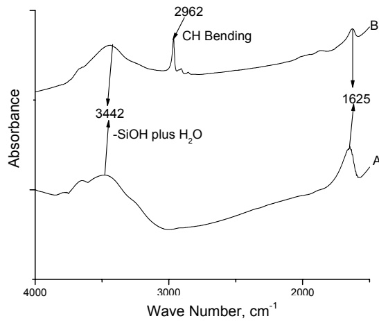
Fig. 1. Infrared spectra: unmodified mesoporous silica (A); TMCS silylated mesoporous silica (B).
