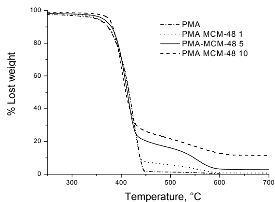
Fig. 4. Thermal degradation of pure PMA and nanohybrids prepared with mesoporous silica.
