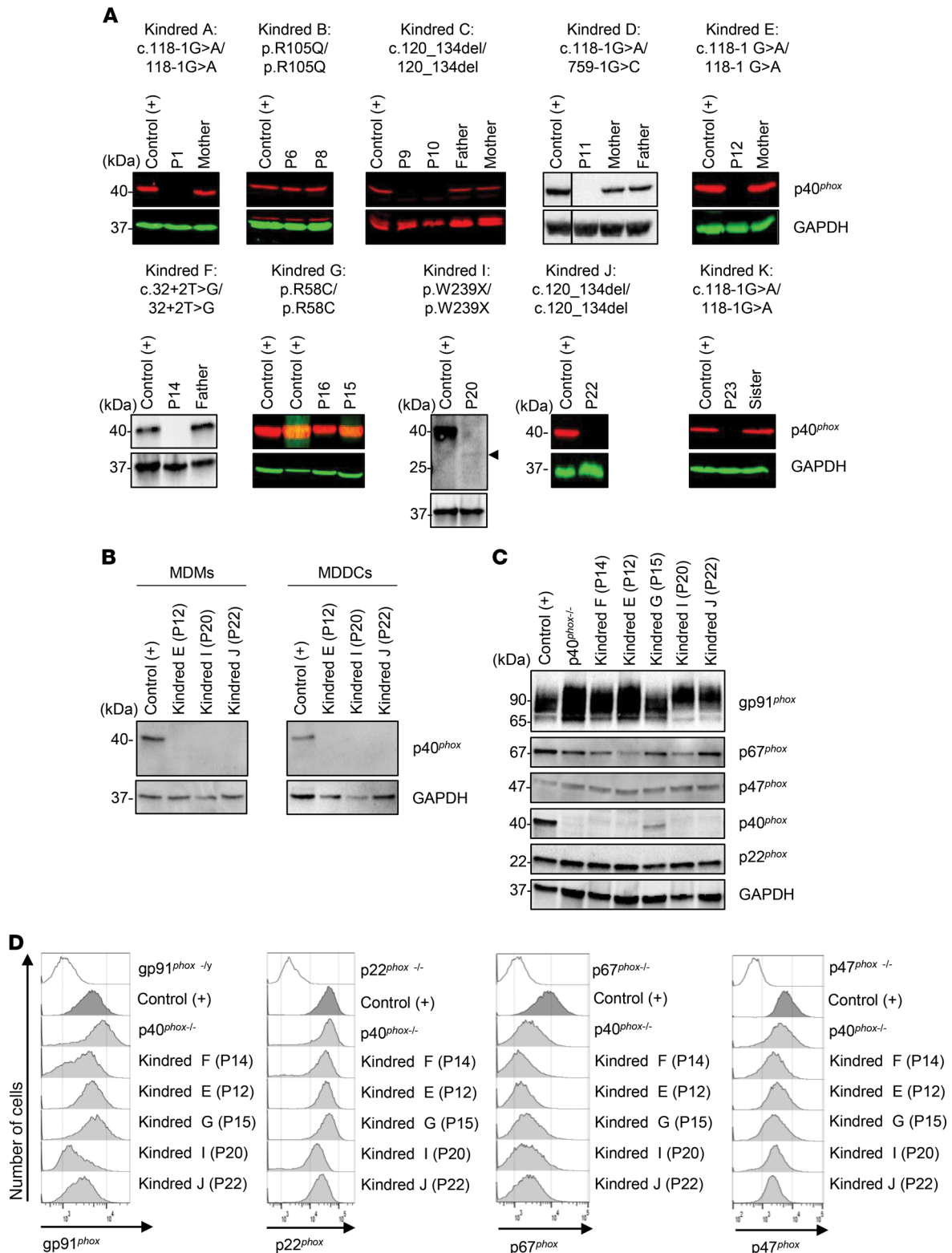
Figure 3. p40 phox and NADPH oxidase subunit expression in p40 phox -deficient cells. (A) Western blot of total protein extracts from the neutrophils of healthy controls, patients, and heterozygous relatives. Abs against p40 phox protein were used. Actin or GAPDH protein was used as a loading control. (B) Western blot of total protein extracts from MDMs and MDDCs from a healthy control and p40 phox -deficient patients. Detection was done with a polyclonal anti-p40 phox Ab, and an Ab against GAPDH was used as a loading control. (C) Western blot of total extracts from EBV-B cells from a healthy control, p40 phox -deficient patients, and XR and AR CGD patients. Abs against p40 phox protein or gp91 phox , p22 phox , p67 phox , and p47 phox were used. Actin or GAPDH protein was used as a loading control. (D) Intracellular detection of gp91 phox , p22 phox , p67 phox , and p47 phox in EBV-B cells from a healthy control, p40 phox -deficient patients, and XR and AR CGD patients. The results shown are representative of 2 independent assays. p40 phox -/- indicates a patient reported in a previous study (26).
