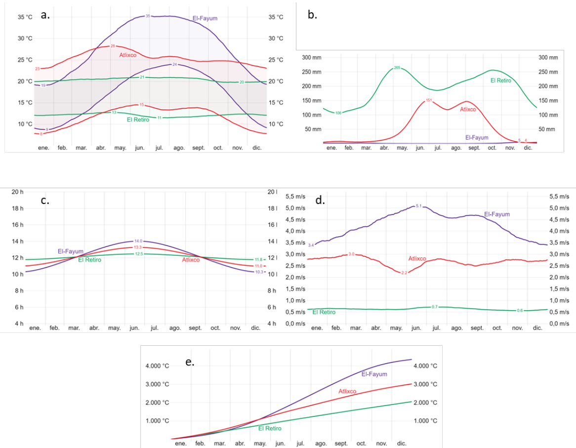
Figure S1. Average monthly climatic conditions of the cultivation areas of the commercial products of Mentha spicata L. evaluated. a. Average maximum and minimum temperature; b. Average monthly rain precipitation; c. Average daylight hours; d. Average monthly wind speed; and e. Cumulative average growing degree days are defined as the thermal integral with a base temperature of 10 °C.
