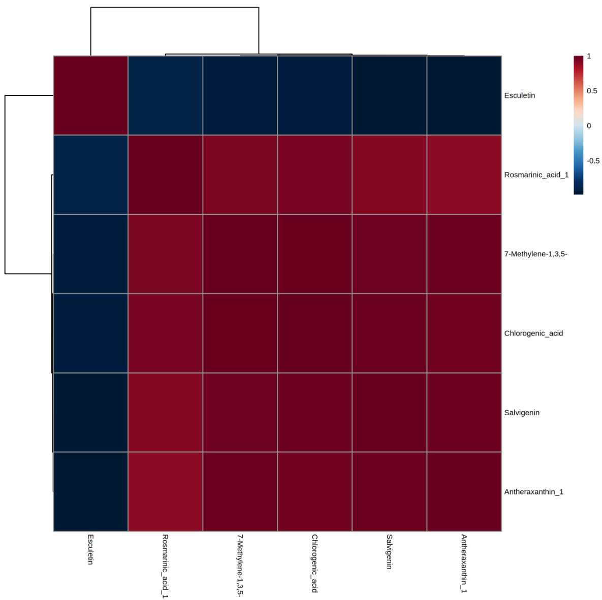
Figure 2. Pearson correlation analysis of the top 6 discriminant metabolites in commercial Mentha spicata samples.
