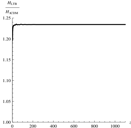
FIG. 3: The ratio between the Hubble parameter H^{LTB}(z) and H^{ACDM}(z) is plotted as function of the redshift for K_0=-0.9376 . The thick lines correspond to the part after the apparent horizon.
