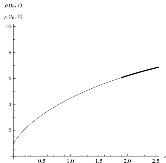
FIG. 4: The energy density profile \frac{\rho(r, t_0)}{\rho(r \rightarrow 0, t_0)} is plotted as function of the comoving radius for K_0=-0.9376 . The thick lines correspond to the part after the apparent horizon.
