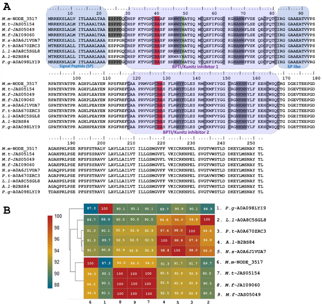
Figure 2. Analysis of the putative long KSPIs identified in the M. mipartitus transcriptome. (A) Deduced amino acid sequence alignment of long Kunitz M.m-NODE-3517 (accession number PP439991) found in M. mipartitus transcriptome with related sequences from public databases ( M. tener ( M.t ), M. fulvius ( M.f ), Notechis scutatus ( N.s ), Pseudonaja textilis ( P.t ), Austrelaps labialis ( A.l ), Laticauda laticadus ( L.l ), and Pantherophis guttatus ( P.g )). The signal peptide and double Kunitz domains are highlighted by colored backgrounds. Active site residues are indicated in red, and N-linked glycosylation in position 46 is indicated in green. Cysteines and the block of hydrophilic aa residues are indicated in gray. (B) Pairwise sequence similarity is highlighted according to percent identity shown in the left-hand column.
