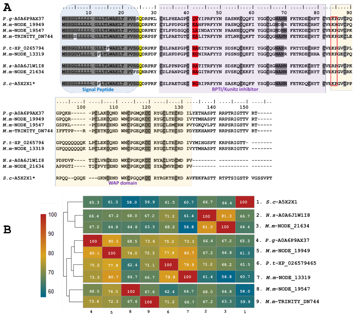
Figure 3. Analysis of the putative Ku-WAP fusin sequences identified in M. mipartitus transcriptome ( M.m -NODE-13319, PP439993; M.m -NODE-19949, PP439992; M.m -NODE-19547, PP439994; M.m -NODE-21634, PP439996; and M.m -TRINITY-DN744, PP439995). (A) Deduced amino acid sequence alignment of the Ku-WAP fusin sequences found in M. mipartitus with related sequences from public databases ( Pantherophis guttatus ( P.g ), Pseudonaja textilis ( P.t ), Sistrurus catenatus edwardsii ( S.c ), and Notechis scutatus ( N.s )). * Ku-WAP fusin identified in viperids with loss of second cystein residue of the WAP domain. The different domains are highlighted by colored backgrounds. The modified residue in position 25 (Q- Pyrrolidone carboxylic acid) is depicted in yellow, the active site at positions 41–42 is depicted in red, and the red box indicates the potential cleavage site between Kunitz and WAP domains in Ku-WAP-fusin. Cysteines and the block of hydrophilic aa residues are indicated in gray. (B) Pairwise sequence similarity is highlighted according to percent identity shown in the left-hand column.
