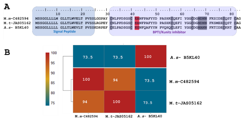
Figure 1. Analysis of the putative short KSPIs identified in the M. mipartitus transcriptome. (A) Deduced amino acid sequence alignment of short Kunitz M.m -C482594 (accession number: PP439990) found in the M. mipartitus transcriptome with related sequences from public databases ( Micrurus tener ( M.t ) and Austrelaps superbis ( A.s )). Colored backgrounds indicate the signal peptide and Kunitz domains. Active site residues are indicated in red. Cysteines and the block of hydrophilic aa residues are indicated in gray. (B) Pairwise sequence similarity is highlighted according to the percent identity shown in the left-hand column.
