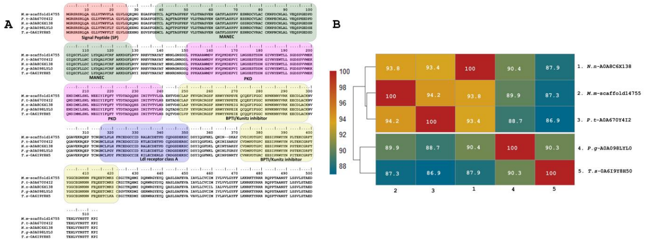
Figure 5. Deduced amino acid sequence alignment of multidomain putative protein ( M.m -scaffold14755, PP439997) annotated as Kunitz identified in the M. mipartitus transcriptome with related sequences published in the database (A). Pairwise sequence similarity is highlighted according to percent identity shown in the left-hand column (B). The signal peptide is indicated in red. Active sites for each Kunitz domain are indicated as RG and EE residues. Micrurus mipartitus ( M.m ), Pseudonaja textilis ( P.t ), Naja naja ( N.n ), Pantherophis guttatus ( P.g ), and Thamnophis sirtalis ( T.s ).
