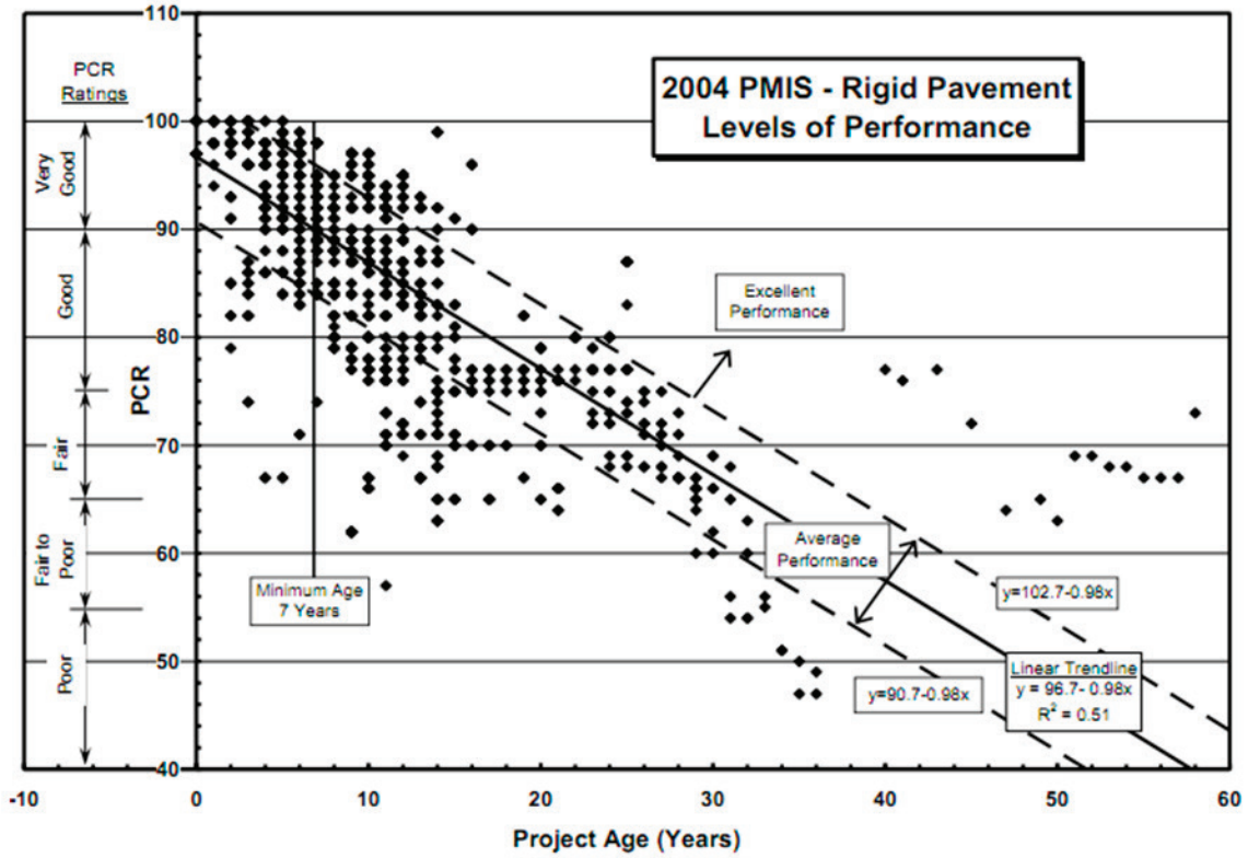
Figure 2. Pavement Condition Rating (PCR) for Rigid Pavements in Ohio. Source Chou et al. [7].
