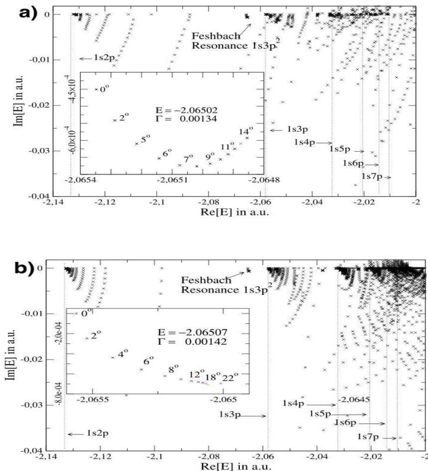
Figura 2. \text{He}^- 4P_e complex eigenvalue spectrum computed with a) Hylleraas CI. b) classical CI. In the insets, the stabilization of the resonance location by varying the rotation angle \theta is shown. Resonance parameters are taken where \partial E/\partial\theta approaches a minimum.
