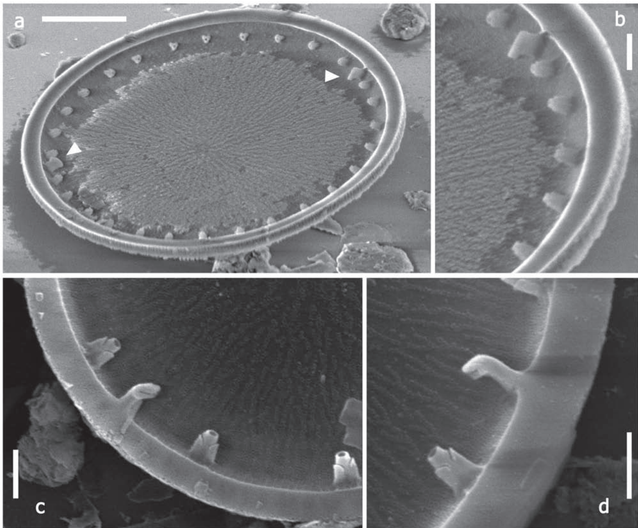
Figure 4. A-D. Internal view of materials from La Fe reservoir, Colombia. SEM. A. Valve view of a tilted specimen. Arrowheads indicate the position of rimoportulae. Note internal openings of fultoportulae surrounded by three satellite pores. B-D. Detail of valve margin showing different internal openings of the rimoportulae (scale bars = 5 \mu\text{m} in A; 1 \mu\text{m} in B-D)
