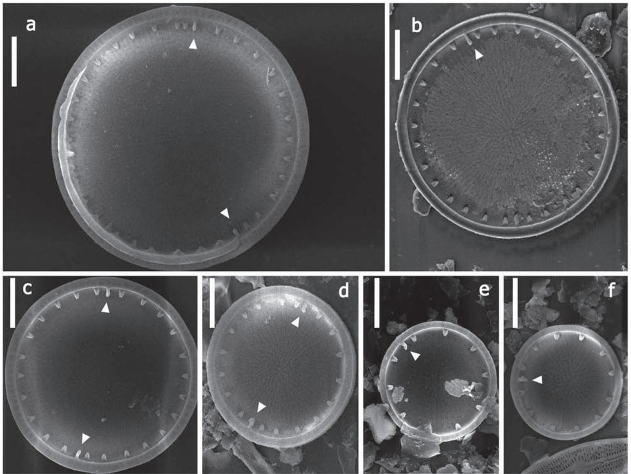
Figure 3. A-F. Internal valve view of different sized specimens from La Fe reservoir, Colombia. SEM. Arrowheads indicate the position of rimoportulae (scale bar = 5 \mu m for all figures)
