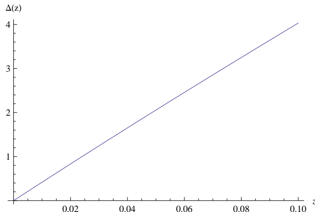
Figure 1. The percentual error \Delta = 100 \frac{D^{\Lambda CDM} - D_{Taylor}^{\Lambda CDM}}{D^{\Lambda CDM}} for a third order expansion is plotted as a function of the redshift. As it can be seen the error is already quite large at redshift 0.1. Higher order expansion does not improve the convergence.
