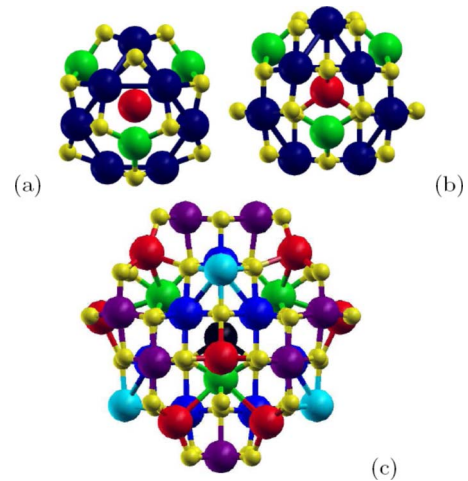
FIG. 1. (Color online) Optimized structures and valence electric charge distribution of the relaxed clusters originated from symmetry Fd\bar{3}m corresponding to (a) C33F , (b) C45F , and (c) C113F . Light gray (yellow) small balls correspond to oxygens, black (dark blue) for \text{Fe}_B ions (and dark gray (purple) in the case of C113F ), whereas \text{Fe}_A ions are represented by light gray (green) and (gray) red spheres (and a central black sphere in the case of C113F ). Different colors correspond also to different charge and magnetization per atom values as described in Tables IV, VI, and VIII.
