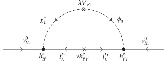
FIGURE 1: Generation of the neutrino masses via the one loop radiative mechanism in the 3-3-1 model with exotic electrons.
