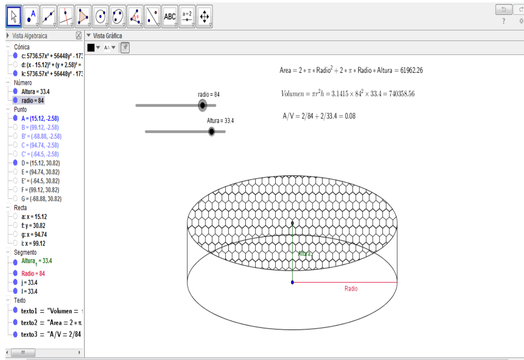
Figure 4. Ratio A/V and its dependence on the values of radius and height.
