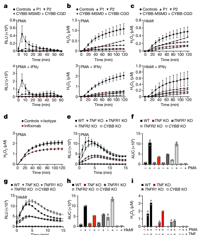
Fig. 3 | Reduced NADPH oxidase activity in TNF-deficient GM-CSF-matured macrophages. a , The production of O 2 - , in relative luminescence units (RLU), by MDMs matured in the presence of GM-CSF for healthy controls ( n = 5 ), patients with TNF deficiency (P1, P2) and patients with variants in CYBB underlying MSMD ( n = 1 ) or CGD ( n = 1 ), after stimulation with PMA with or without IFN \gamma . Data of healthy controls ( n = 5 ) are mean \pm s.d. b, c , The extracellular production of H 2 O 2 in GM-CSF-matured MDMs for healthy controls ( n = 5 ), patients with TNF deficiency (P1 and P2) and patients with variants in CYBB underlying MSMD ( n = 1 ) or CGD ( n = 1 ), after stimulation with PMA ( b ) or in response to serum-opsonized heat-killed M. tuberculosis (HkMt) ( c ) with or without IFN \gamma . Data of healthy controls ( n = 5 ) are mean \pm s.d. d , H 2 O 2 release by GM-CSF-matured MDMs from healthy controls differentiated in culture medium in the presence of infliximab or the corresponding isotype control. One representative experiment of two independent experiments with three biological replicates. Data are mean \pm s.d. e , O 2 - production in response to PMA stimulation by iPS-cell-derived macrophages and iPS-cell-derived macrophages gene-edited to KO TNF , TNFR1 , TNFR2 or CYBB expression. One representative experiment of three independent experiments with three biological replicates. Data are mean \pm s.d. f , Area-under-the-curve (AUC) analysis of O 2 - production by iPS-cell-derived macrophages as in e with or without PMA stimulation. Data are mean \pm s.d. of three independent experiments. g , O 2 - production by iPS-cell-derived macrophages in response to stimulation with heat-killed M. tuberculosis . One representative experiment of three independent experiments with three biological replicates. Data are mean \pm s.d. h , AUC analysis of O 2 - production by iPS-cell-derived macrophages as in g with or without stimulation with heat-killed M. tuberculosis . Data are mean \pm s.d. of three independent experiments. i , Extracellular H 2 O 2 release by iPS-cell-derived macrophages in response to PMA with or without TNF. n = 2 independent experiments.
