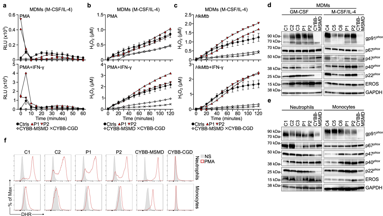
Extended Data Fig. 7 | NADPH oxidase expression and activity in TNF-deficient phagocytes. a , Production of O_2^- , in relative luminescence units (RLU), by MDMs matured in the presence of M-CSF and IL-4, for healthy controls ( n = 5 ), TNF-deficient patients, and patients with variants in CYBB underlying MSMD ( n = 1 ) or CGD ( n = 1 ) after stimulation with PMA with or without IFN- \gamma . For healthy controls ( n = 5 ) the data are mean \pm s.d. b , Extracellular production of H_2O_2 in M-CSF/IL-4-matured MDMs as in ( a ) after stimulation with PMA with or without IFN- \gamma . Data are mean \pm s.d. c , H_2O_2 release by M-CSF/IL-4-matured MDMs as in ( a ) in response to serum-opsonized heat-killed Mtb ( HkMtb ) stimulation with or without IFN- \gamma . Data are mean \pm s.d. d , Western blot of whole-
