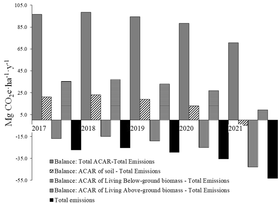
Fig. 3 Carbon balance (Emissions–Removals or ACAR) per year at Villa Lucero farm in the Colombian Amazon, considering 4 scenarios: total ACAR, soil ACAR, aboveground biomass ACAR, and belowground biomass ACAR
